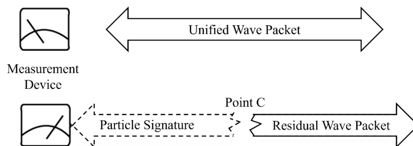
Figure 1: Fracture of a Unified Wave Packet Constrained by Conservation Laws
